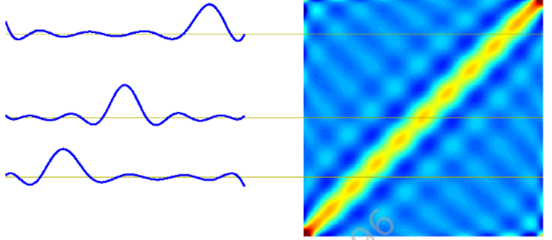
Figure 3.10 The equivalent kernel k(x, x') for the Gaussian basis functions in Figure 3.1, shown as a plot of x versus x' , together with three slices through this matrix corresponding to three different values of x . The data set used to generate this kernel comprised 200 values of x equally spaced over the interval (-1, 1) .
