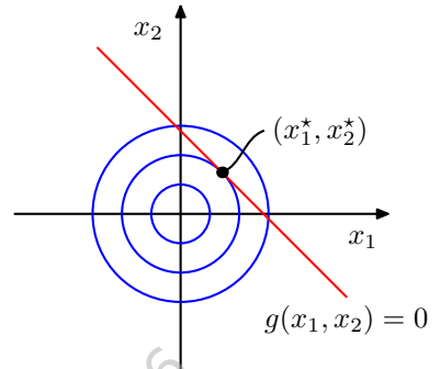
Figure E.2 A simple example of the use of Lagrange multipliers in which the aim is to maximize f(x_1, x_2) = 1 - x_1^2 - x_2^2 subject to the constraint g(x_1, x_2) = 0 where g(x_1, x_2) = x_1 + x_2 - 1 . The circles show contours of the function f(x_1, x_2) , and the diagonal line shows the constraint surface g(x_1, x_2) = 0 .
