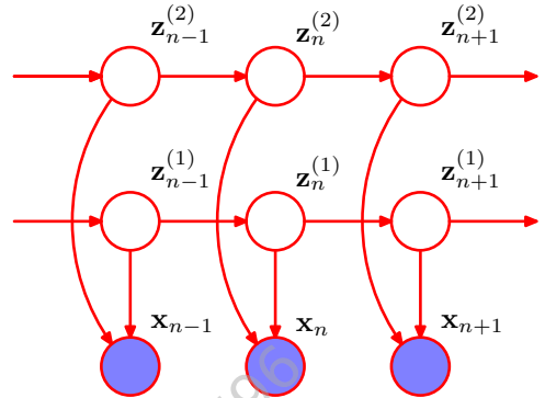
Figure 13.19 A factorial hidden Markov model comprising two Markov chains of latent variables \mathbf{z} , one possible choice of emission model is a linear-Gaussian density in which the mean of the Gaussian is a linear combination of the states of the corresponding latent variables.
