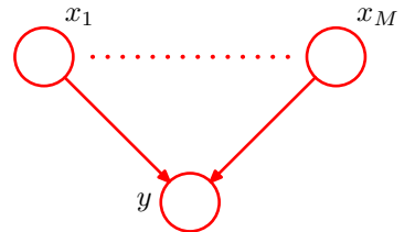
Figure 8.13 A graph comprising M parents x_1, \dots, x_M and a single child y , used to illustrate the idea of parameterized conditional distributions for discrete variables.
